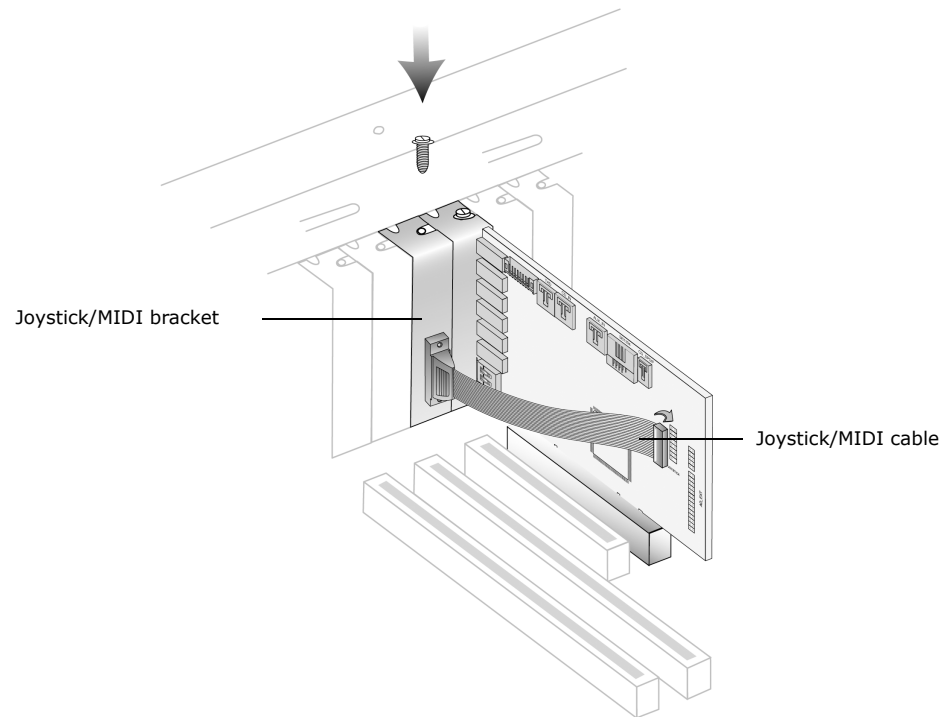
Figure 1-5: Securing the Joystick/MIDI bracket.
