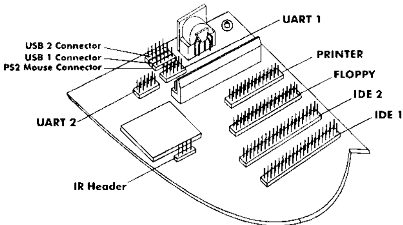
A Part of P51430VX-250 Explorer Main Board
