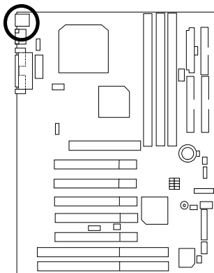
PS/2 Keyboard
